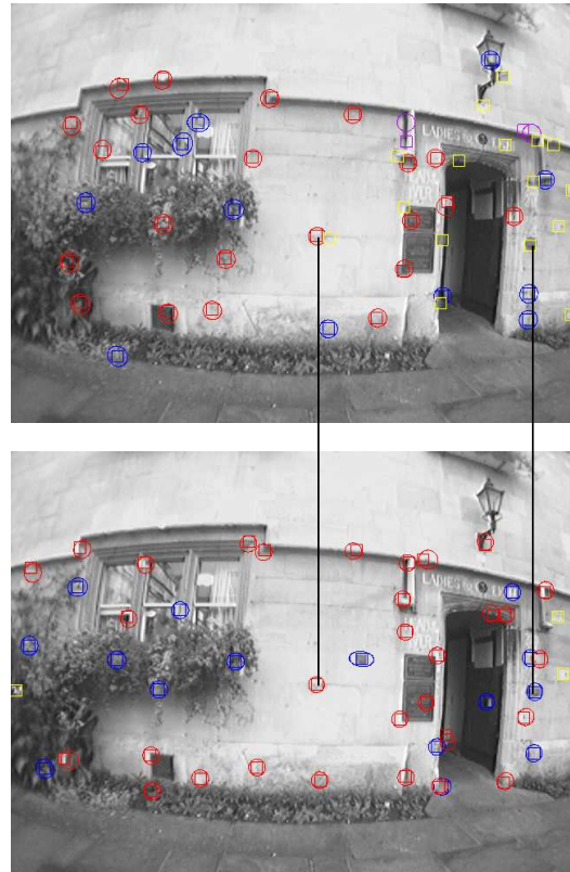
Fig. 3. During the overlap in the sequence, the system tracks the camera in two submaps. The colours indicate if an observation was successful (red), unsuccessful (blue), rejected by JCBB (purple), or not attempted, (yellow). Only two of the visible features are actually common to both submaps.
